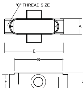
Type X Dimensions (in Inches) – Threaded & Set Screw:
