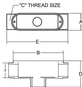
Type TB Dimensions (in Inches) – Threaded & Set Screw:
