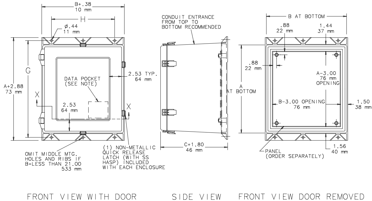
Hinged with Quick-Release Latch Enclosures 36 X 30 or Smaller Drawing
