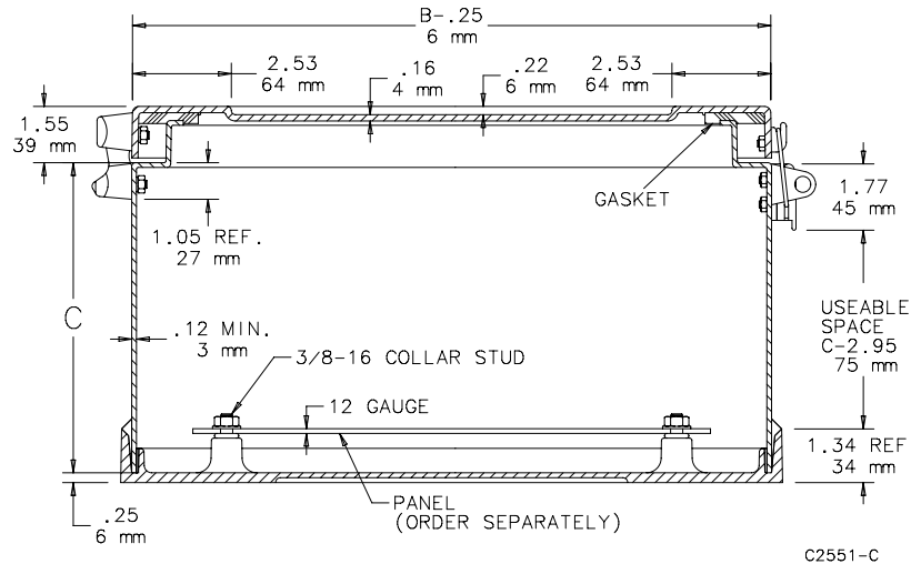
SECTION X-X
