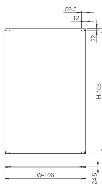
Mounting plate view
