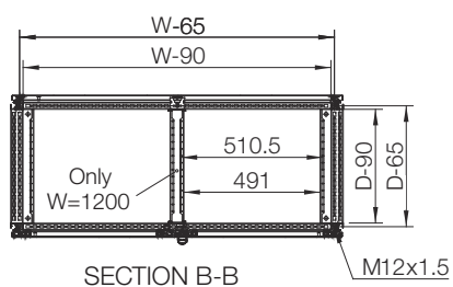
Sectional top view (without bottom plates)
