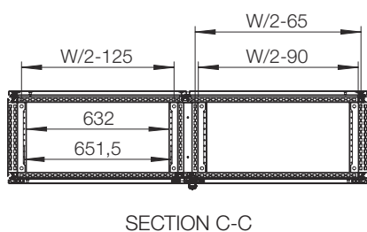
Sectional top view W=1600 (without bottom plates)
